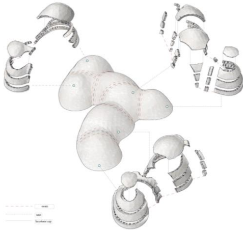
Figure 12. Global sequence: successive units.
