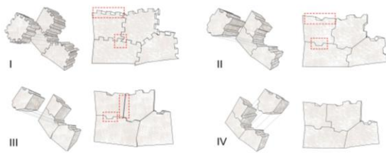
Figure 6. Interlocking system experiments
