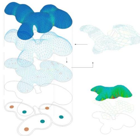
Figure 1. RhinoVault form finding process.
