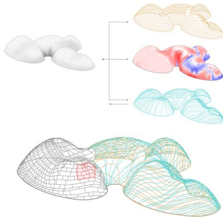
Figure 4. Customised cutting pattern. Selected patch is outlined.
