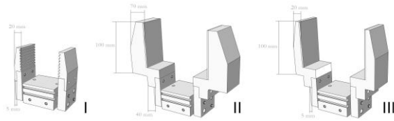
Figure 8. End effector design
