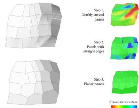
Figure 5. Planarisation. Curvature analysis
