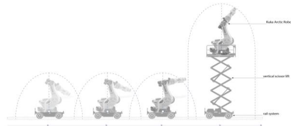
Figure 7. Robotic scissors lift system
